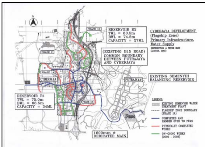
CYBERJAYA DEVELOPMENT (FLAGSHIP ZONE) PRIMARY INFRASTRUCTURE, WATER SUPPLY
